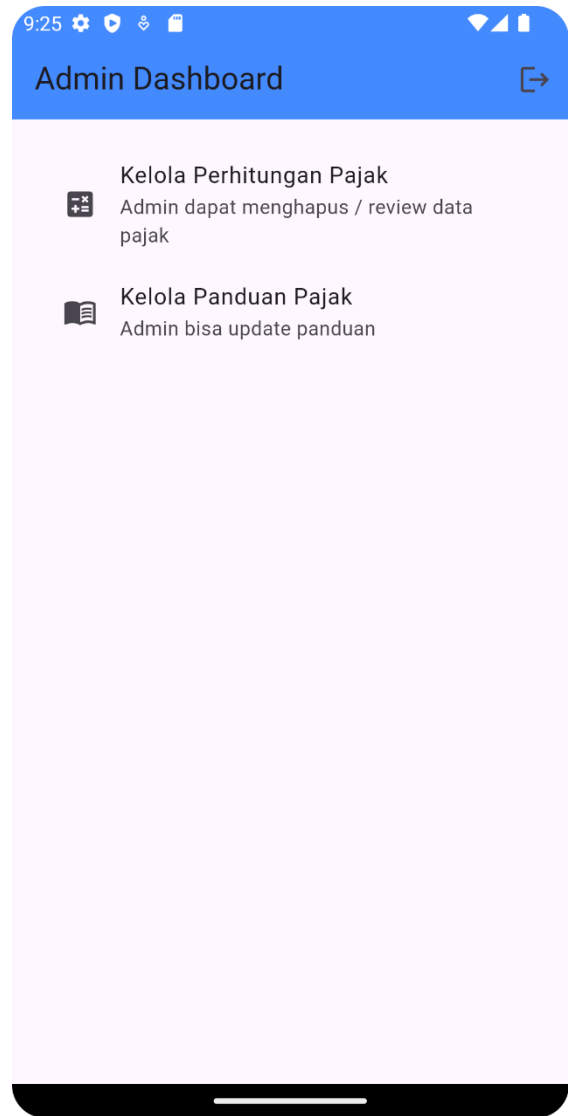
Gambar 4. Dashboard Admin
