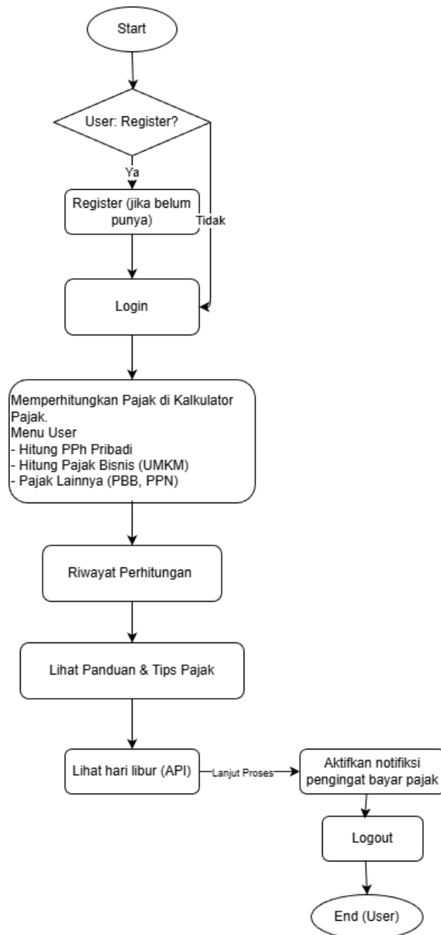
Gambar 2. Flowchart User
