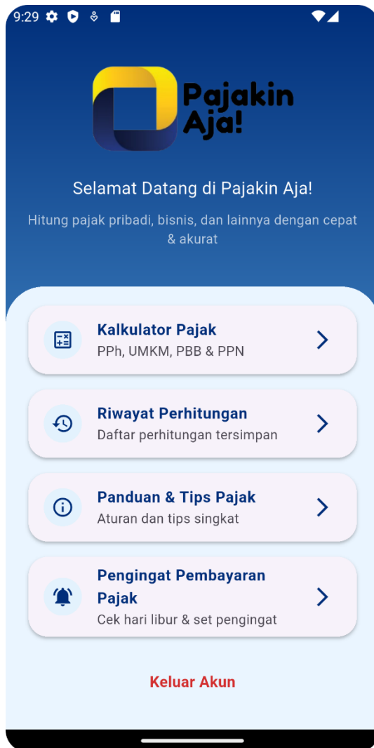
Gambar 9. Halaman User
